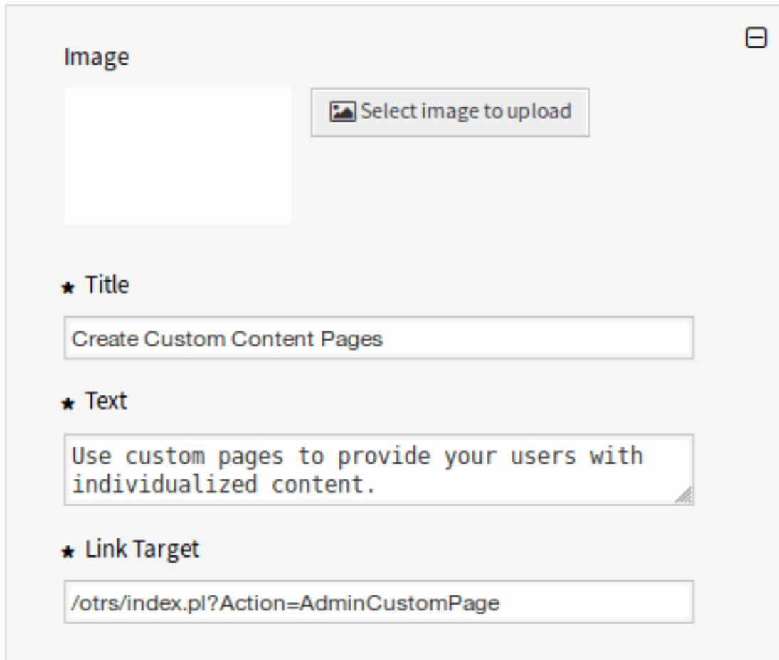
Fig. 6.17: Image Teaser
