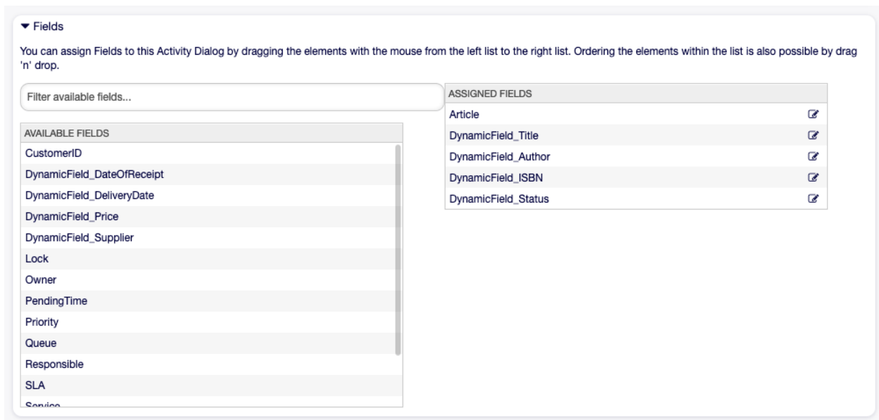
Figure 1.201: Book Ordering - Add Activity Dialog Fields
