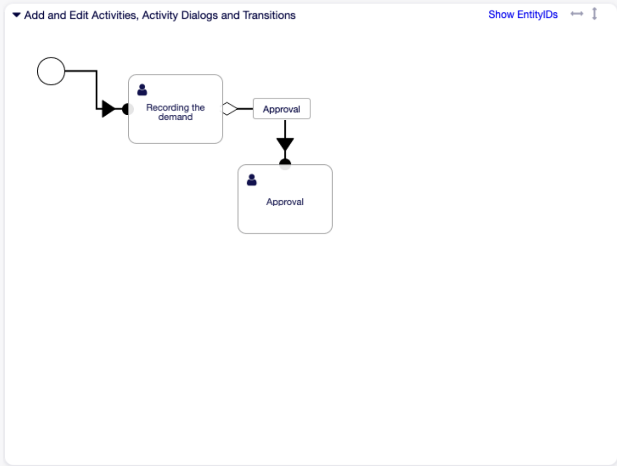
Figure 1.213: Book Ordering - First Transition On Canvas
