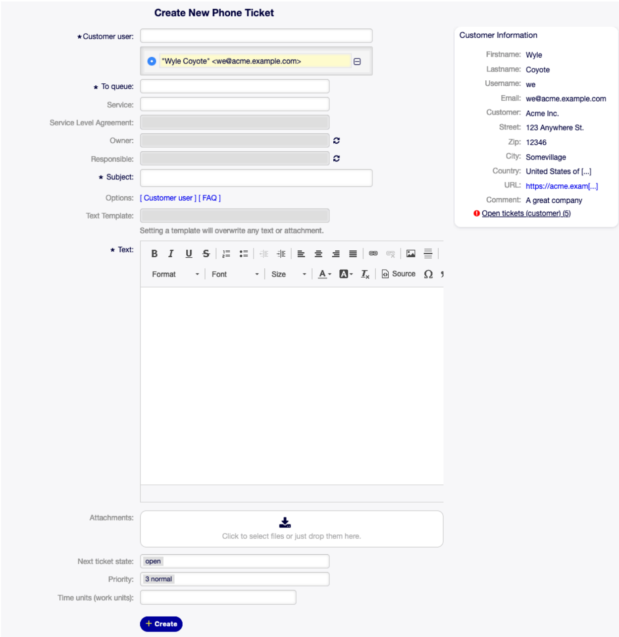
Fig. 6.30: New Phone Ticket Screen
